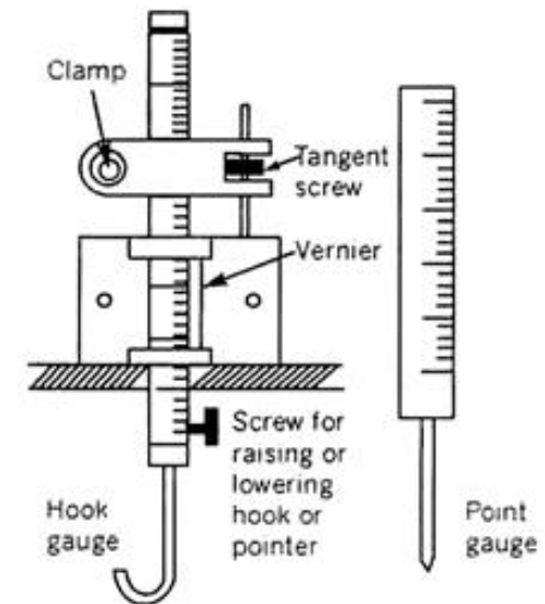
Fig. 15.5. Hook and point gauges.
