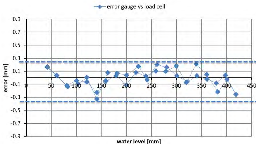
Figure 9. Level measurement error on the hydraulic model TARZOUT [4]
