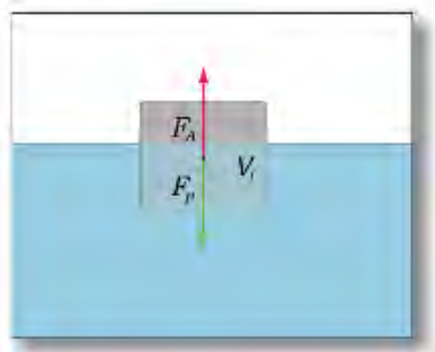
Figure 2. Force equilibrium in a floating solid body [7]
